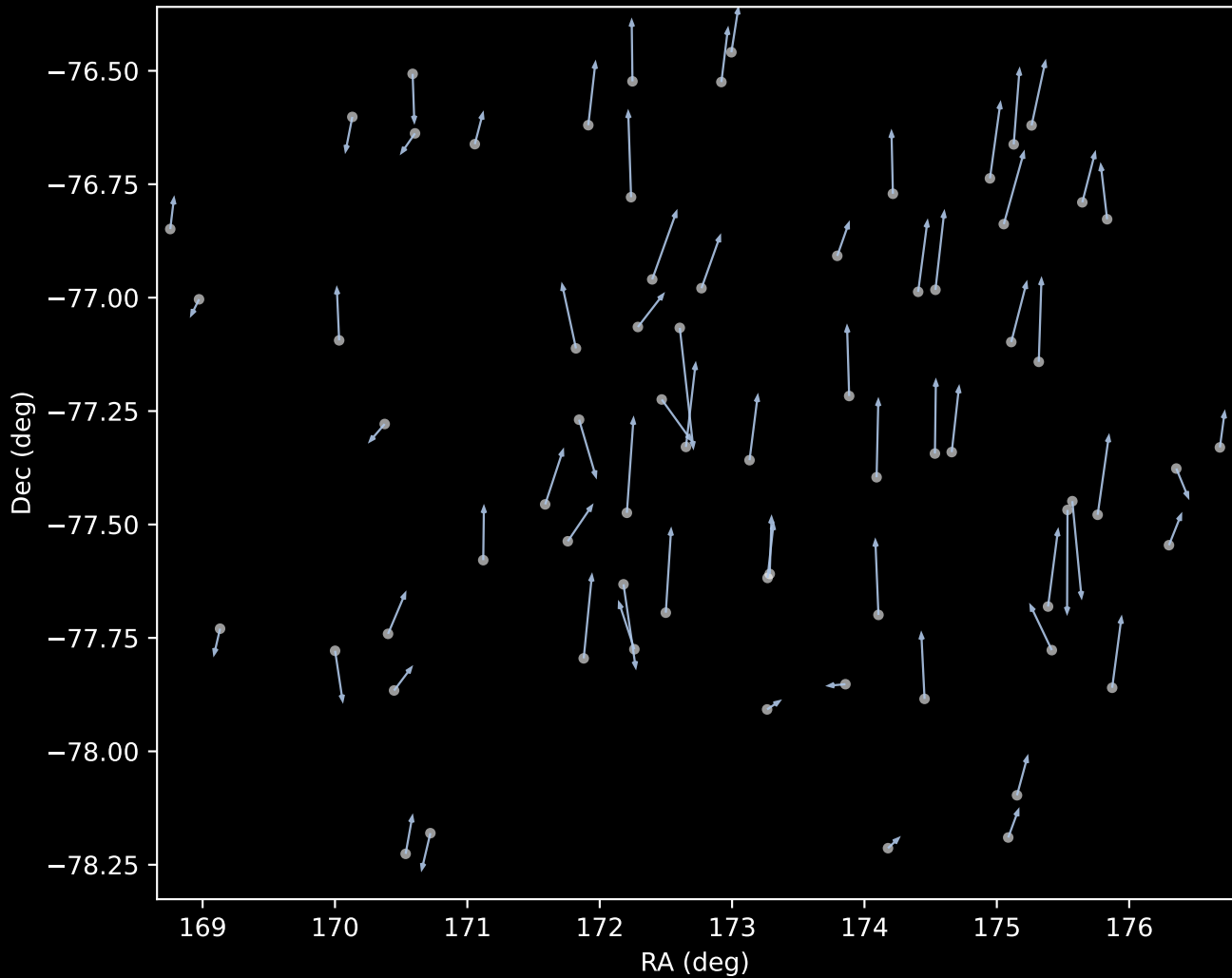
GALAH DR4 Cluster 1 Proper Motion Vectors (n=70)
