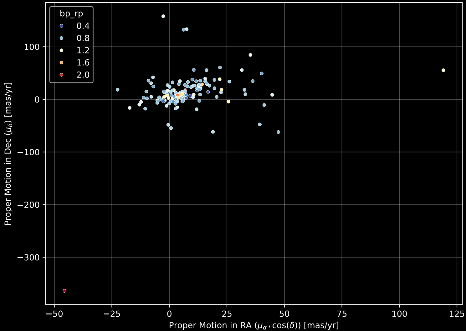
GALAH DR4 Field: [7240] Proper Motion Diagram (n= 145)
