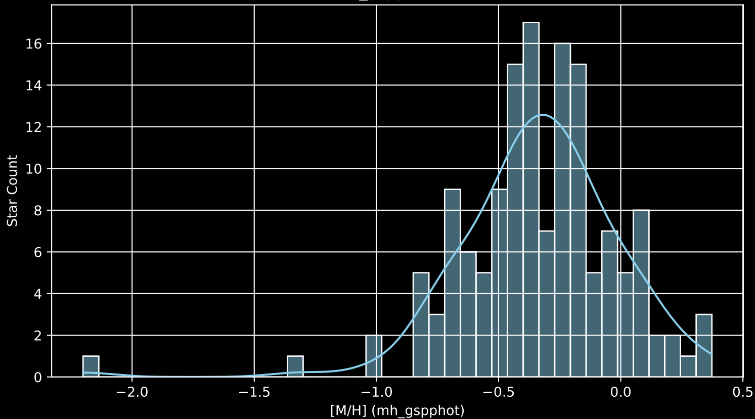
GALAH DR4 Field: [7240] [M/H] (mh_gspphot) (n= 144)
