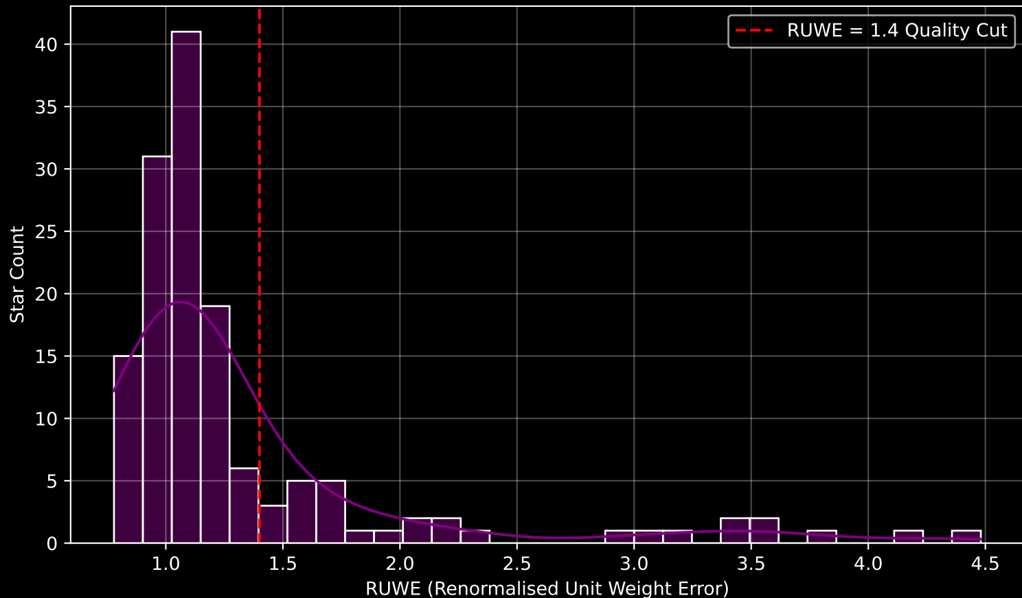
GALAH DR4 Field [7240] RUWE Distribution (n= 142)
