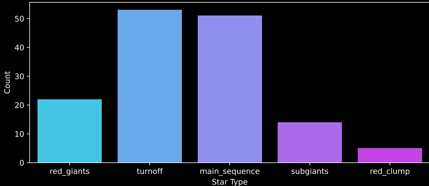
GALAH DR4 Field: [7240] Count plot of Star Type
