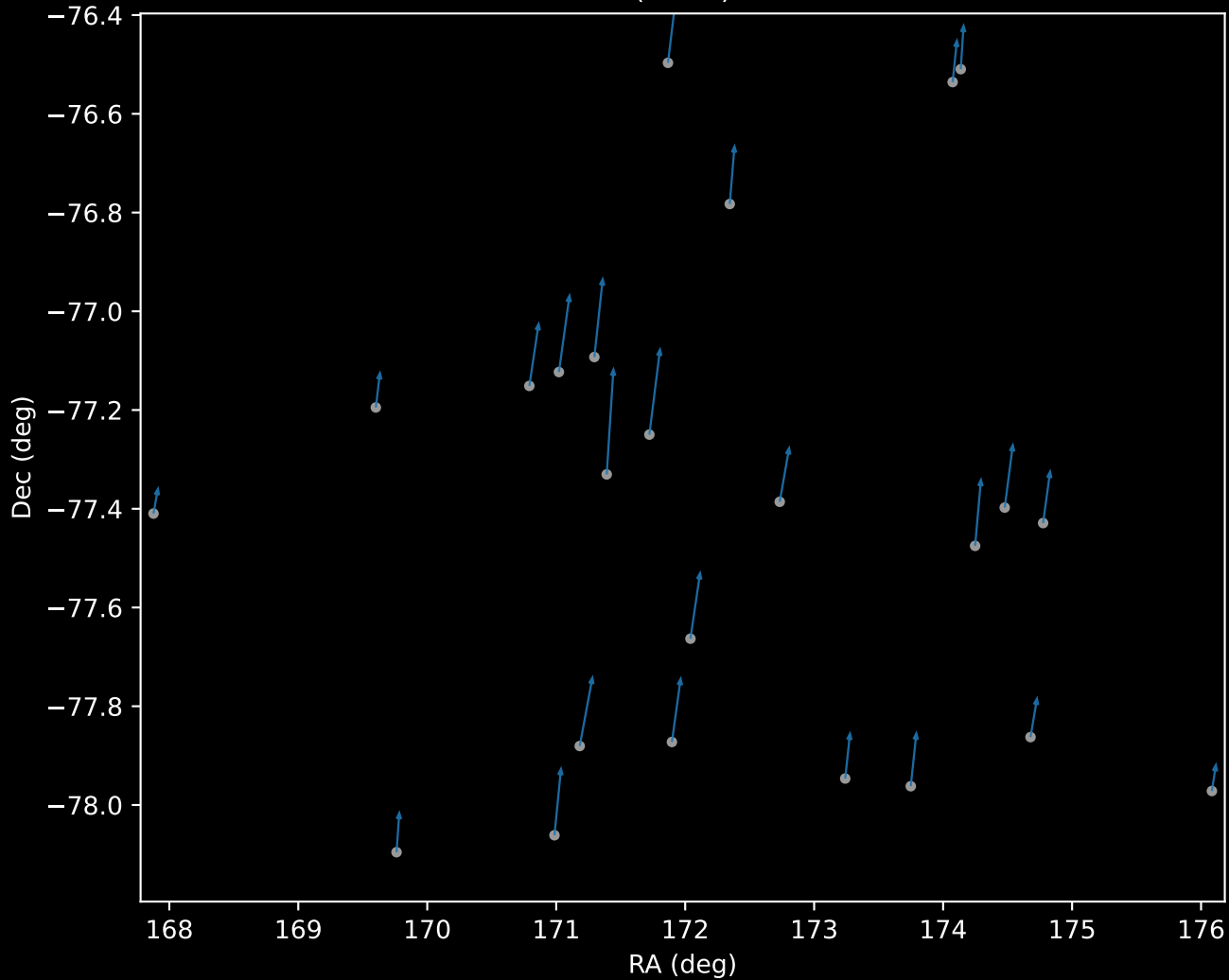
GALAH DR4 Cluster 0 Proper Motion Vectors (n=24)
